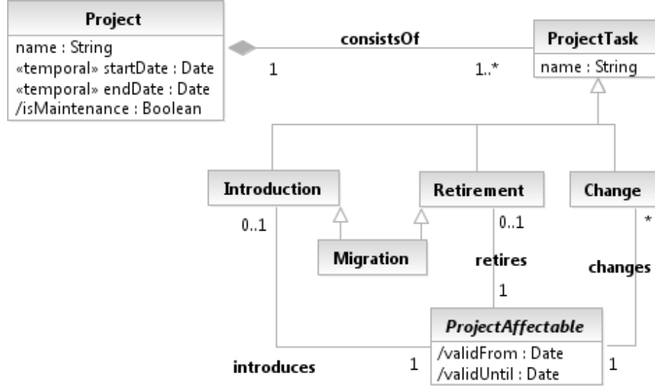
Fig. 3. Project affectable and project with exemplary child class
