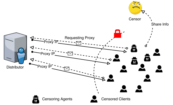
Fig. 1. Proxy distribution (assignment) in a circumvention system.
