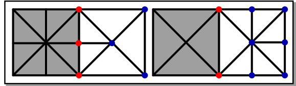
Figure 4: Best and worst cases for vertex cache re-usage of fans. The gray fan can re-use the red vertices of the white fan, resulting in a cache coherence of at least 25%
